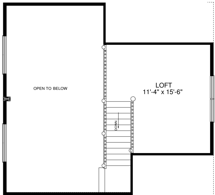
Suggested Second Floor Layout – Work Performed on Site
